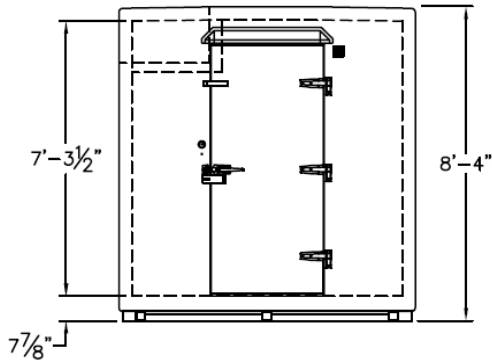
DT810 Elevation View
