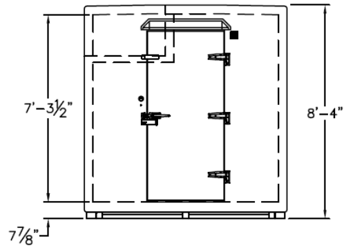
DT820 Elevation View
