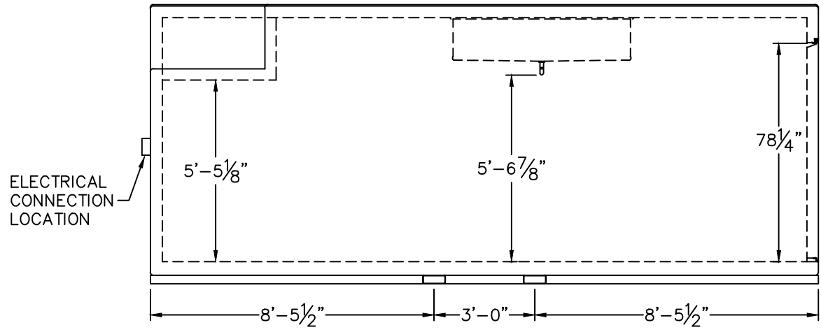
ELEVATION VIEW
