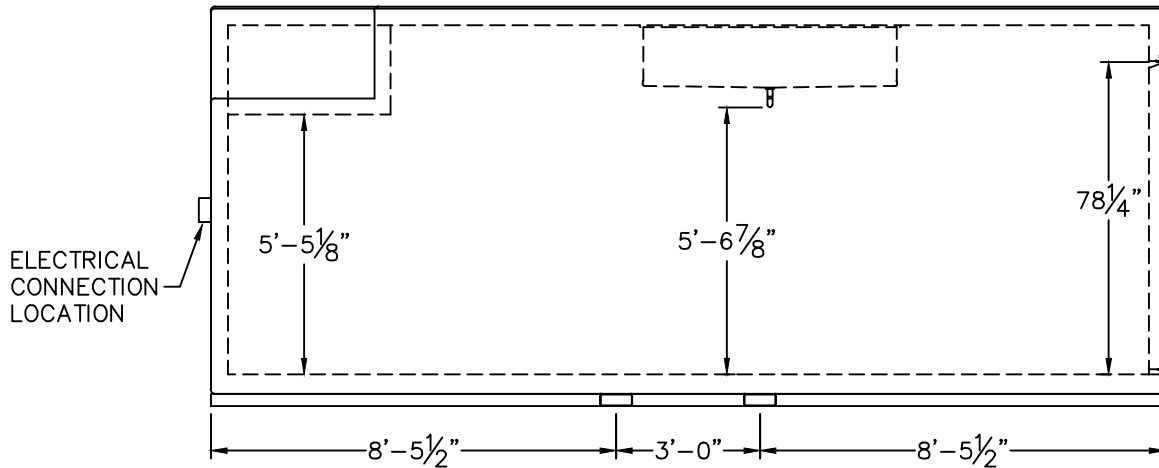
ELEVATION VIEW
